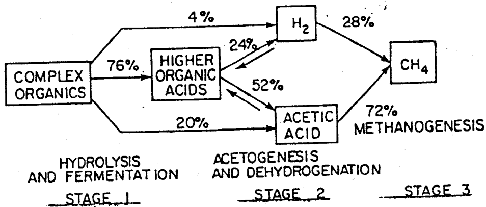
Fig 4.1: The stages of methane fermentation.
