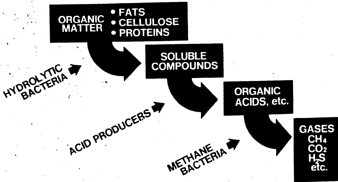
Fig. 9.2. Microbial reactions that occur in anaerobic processes.
